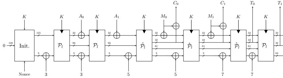
Fig. 3: The Description of TinyJAMBU Mode [23]
