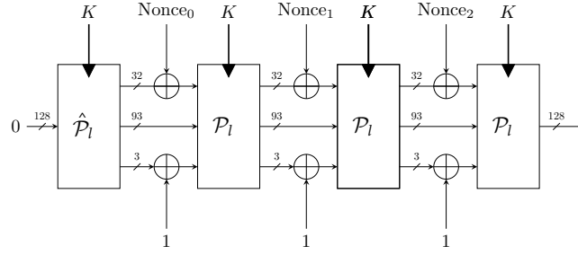
Fig. 2: The Initialization of TinyJAMBU [23]
