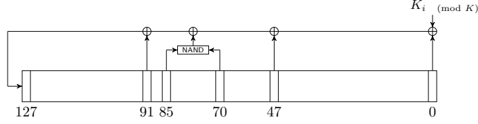
Fig. 1: The Permutation P^{k_i}
