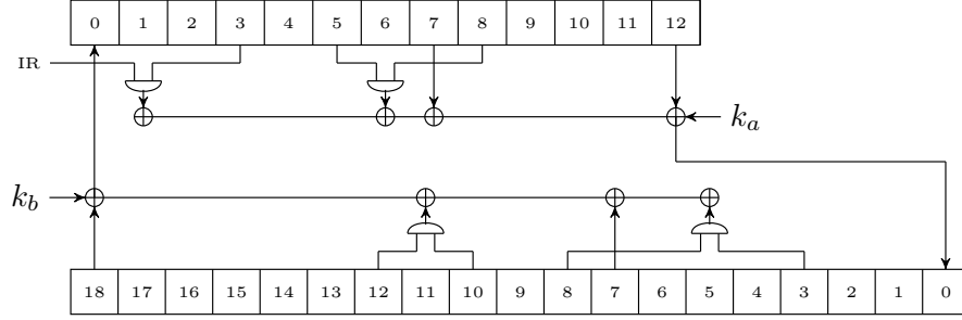
Fig. 4: Round Function of KATAN32
