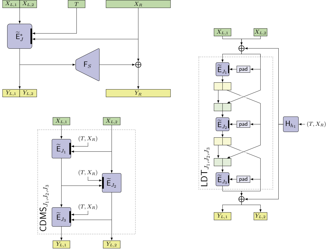
Fig. 10: Top left: Extended UIV construction with a black-box tweakable blockcipher \tilde{E} ; Bottom left: CDMS extender; Right: LRW2 + LDT extender.
