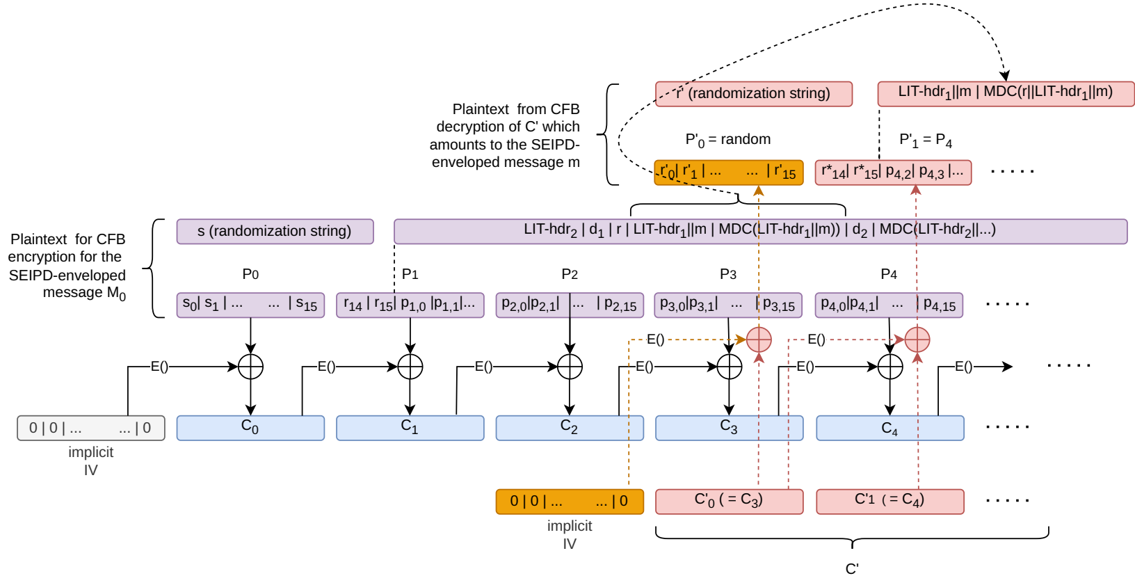
Figure 2: Depiction of an attempted adaptively chosen ciphertext attack against SEIPD encryption assuming a block size of 16 bytes. Here, E() indicates block encryption under the given block cipher key and \oplus denotes XOR. The violet plaintext consisting of the bytes p_{1,0}, p_{1,1}, \dots is the message M_0 prepared by the attacker enveloped in the outer LIT packet with the header LIT-hdr_2 . Above the blocks P_0, P_1, \dots , the semantic interpretation of the decrypted plaintext is depicted in the same color. The light blue boxes show the resulting ciphertext C . The red and orange boxes represent the manipulated ciphertext C' and the plaintext resulting from its decryption. Here the red boxes represent repositioned ciphertext and plaintext blocks and the orange ones entirely different blocks. The red and orange arrows and XOR operators indicate the data flows and operations during decryption of C' . Since, as indicated by the orange boxes, the implicit IV of the all-zero block of the repositioned message is different from the originally preceding cipher block, the attacker cannot predict the value of r' .
