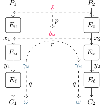
Fig. 2: Building blocks of a DL distinguisher in the sandwich framework.
