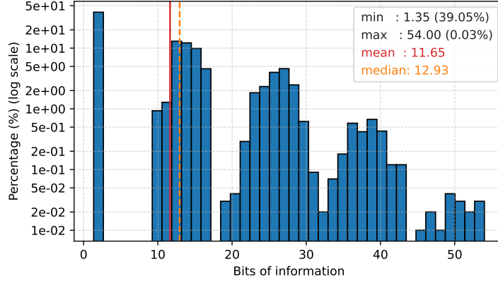
Fig. 6: Histogram of the bit information obtained by four 5-round distinguishers
