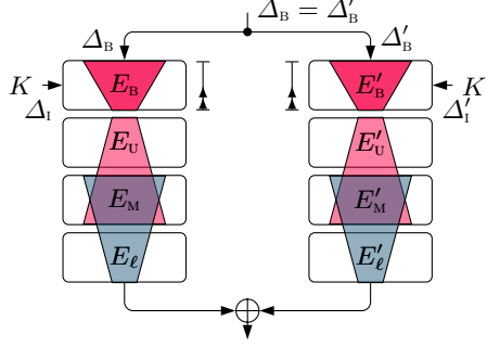
Fig. 4: Full attack setup on SoP designs.
