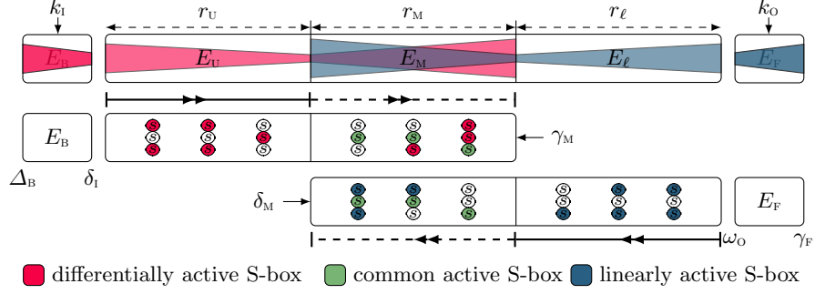
Fig. 3: Searching for complete DL attacks.
