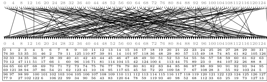
(b) Bit permutation P_{bk2} for the key schedule of Branch2.
