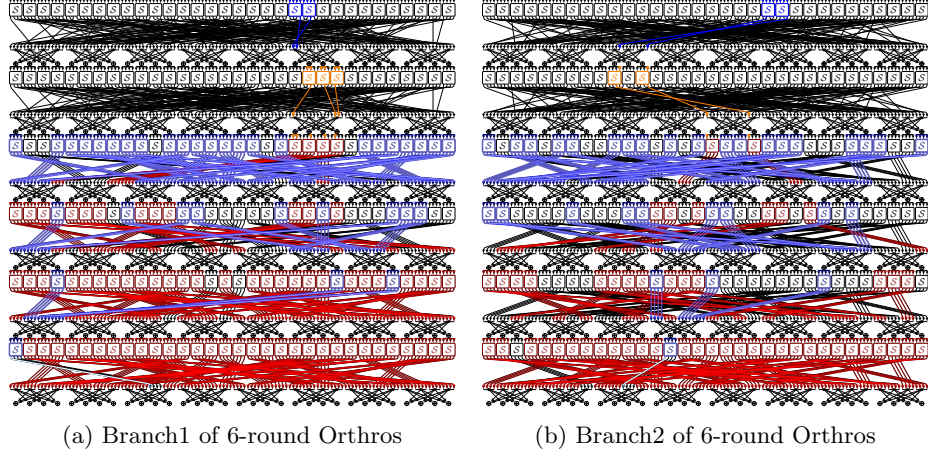
Fig. 31: 6-Round DL Attack 1 on Orthros
