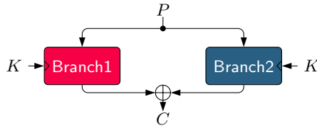
Fig. 9: The Orthros PRF construction.
