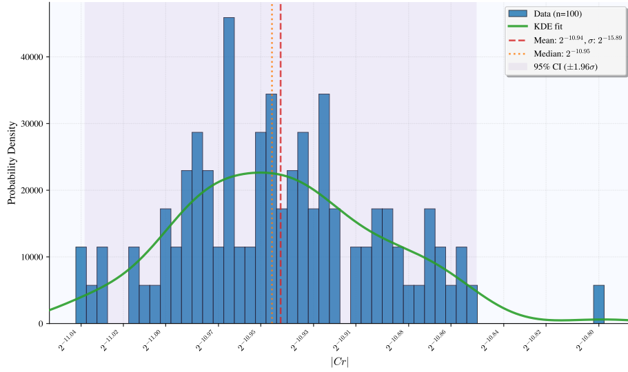
Fig. 29: Empirical correlation distributions for the 5-round distinguisher in Figure 5 (Orthros-PRF), evaluated over 100 random keys with N = 2^{32} samples per key.
