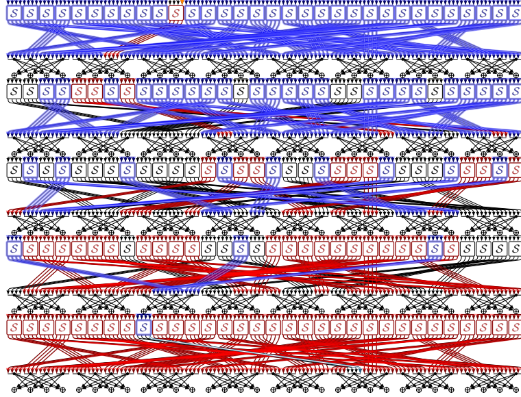
Fig. 21: DL distinguisher for 5 rounds of Branch1 in Orthros
