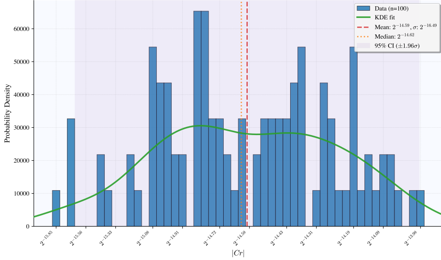
Fig. 30: Empirical correlation distributions for the 5-round distinguisher in Figure 31 (Orthros-PRF), evaluated over 100 random keys with N = 2^{33} samples per key.
