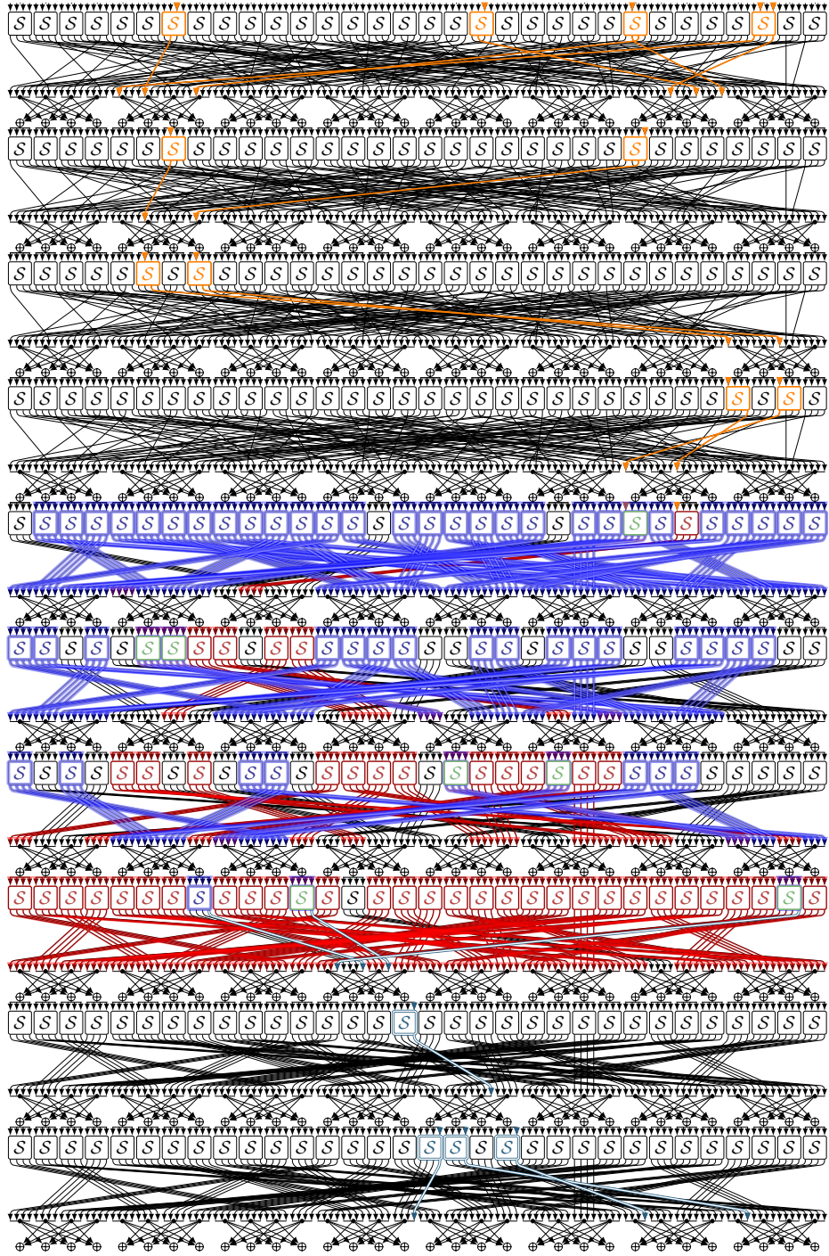
Fig. 24: DL distinguisher for 10 rounds of Branch1 in Orthros
