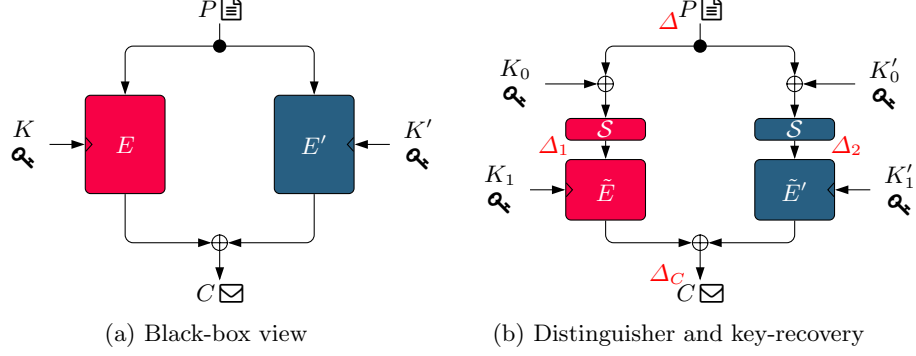
Fig. 1: Weak-key attack problem on sum of permutations.
