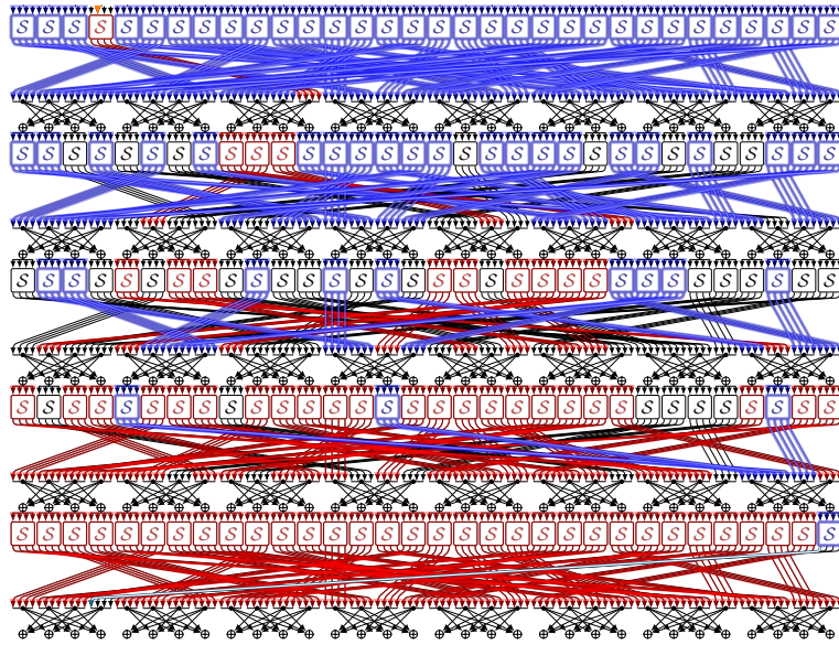
Fig. 25: DL distinguisher for 5 rounds of Branch2 in Orthros
