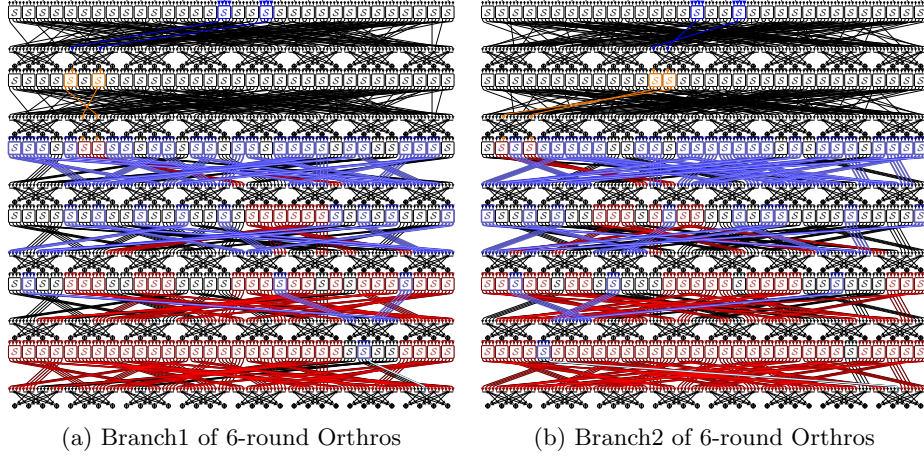
Fig. 5: 6-Round DL attack 0 on Orthros
