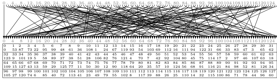
(a) Bit permutation P_{bk1} for the key schedule of Branch1.
