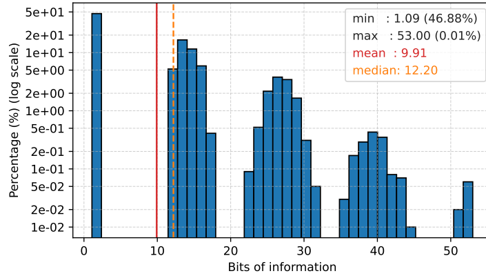
Fig. 7: Histogram of the bit information obtained by four 7-round distinguishers
