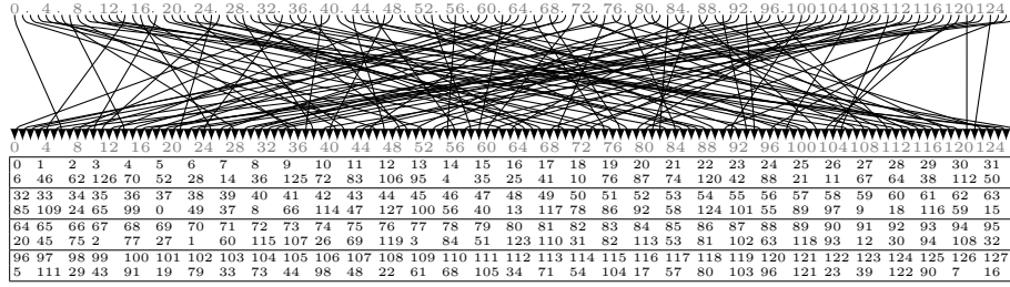
(c) Bit permutation P_{br1} for rounds 5 to 11 of Branch1.
