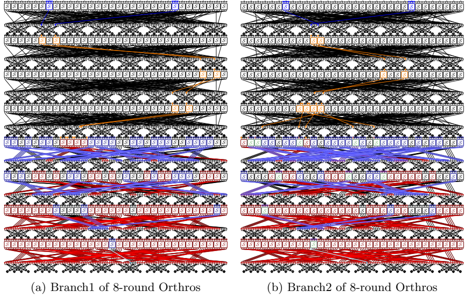
Fig. 36: 8-Round DL Attack 2 on Orthros
