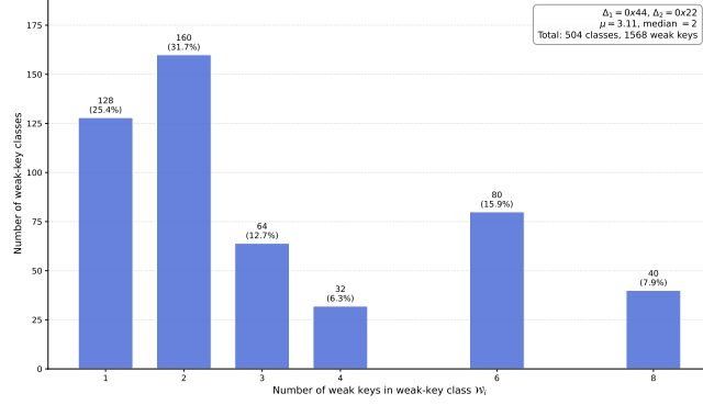
Fig. 8: Weak-key class distribution in Example 1.
