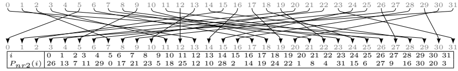
(b) Nibble permutation P_{nr2} for rounds 1 to 4 of Branch2.
