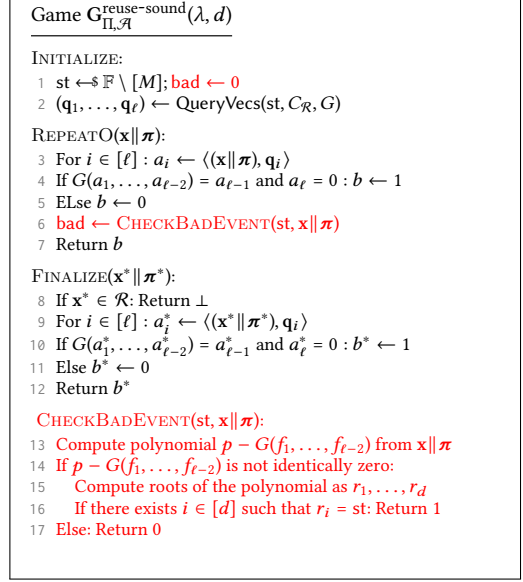
Figure 15: Game defining reusable soundness property for BBG + . Modifications to include a bad flag are given in red.
