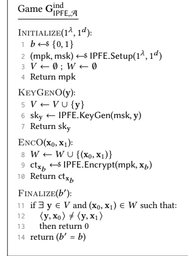
Figure 2: Indistinguishability-based security game for IPFE.
