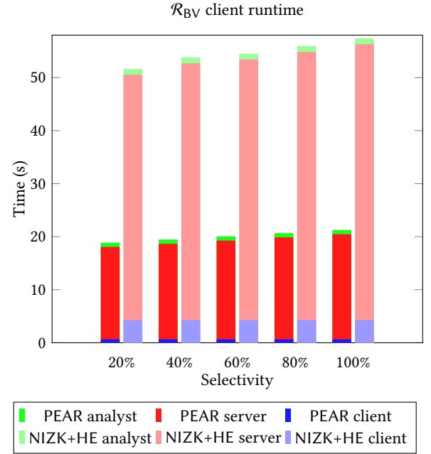
Figure 13: Total runtimes.
