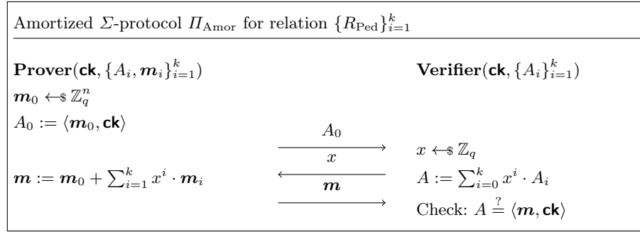
Fig. 1: Procedure of amortized \Sigma -protocol \Pi_{\text{Amor}} .
