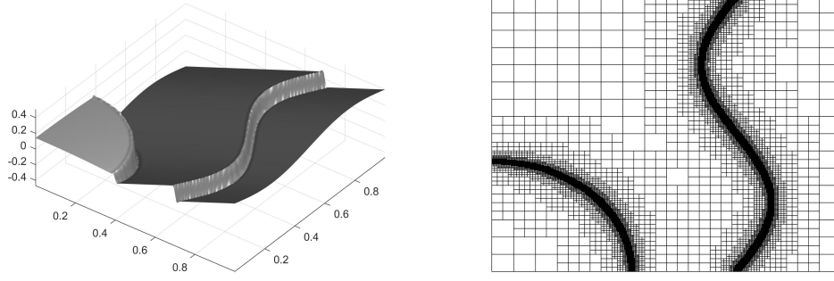
(a) Fault detection-based surface reconstruction (14210 NDOF).
