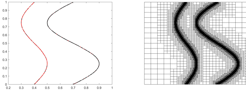
(a) Adaptive refinement based on null rules (20054 NDOF).
