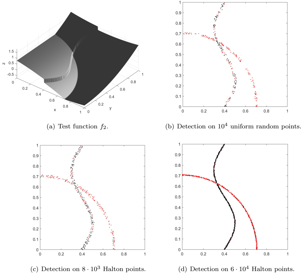
Fig. 2: Application of the detection algorithm on data sampled from the test function f_2 (top left). The results obtained by considering 10^4 uniformly distributed random points (top right), as well as 8 \cdot 10^3 (bottom left) and 6 \cdot 10^4 (bottom right) Halton points are shown.
