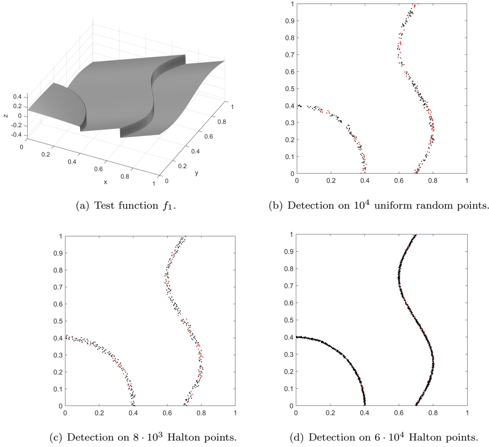
Fig. 1: Application of the detection algorithm on data sampled from the test function f_1 (top left). The results obtained by considering 10^4 uniformly distributed random points (top right), as well as 8 \cdot 10^3 (bottom left) and 6 \cdot 10^4 (bottom right) Halton points are shown.
