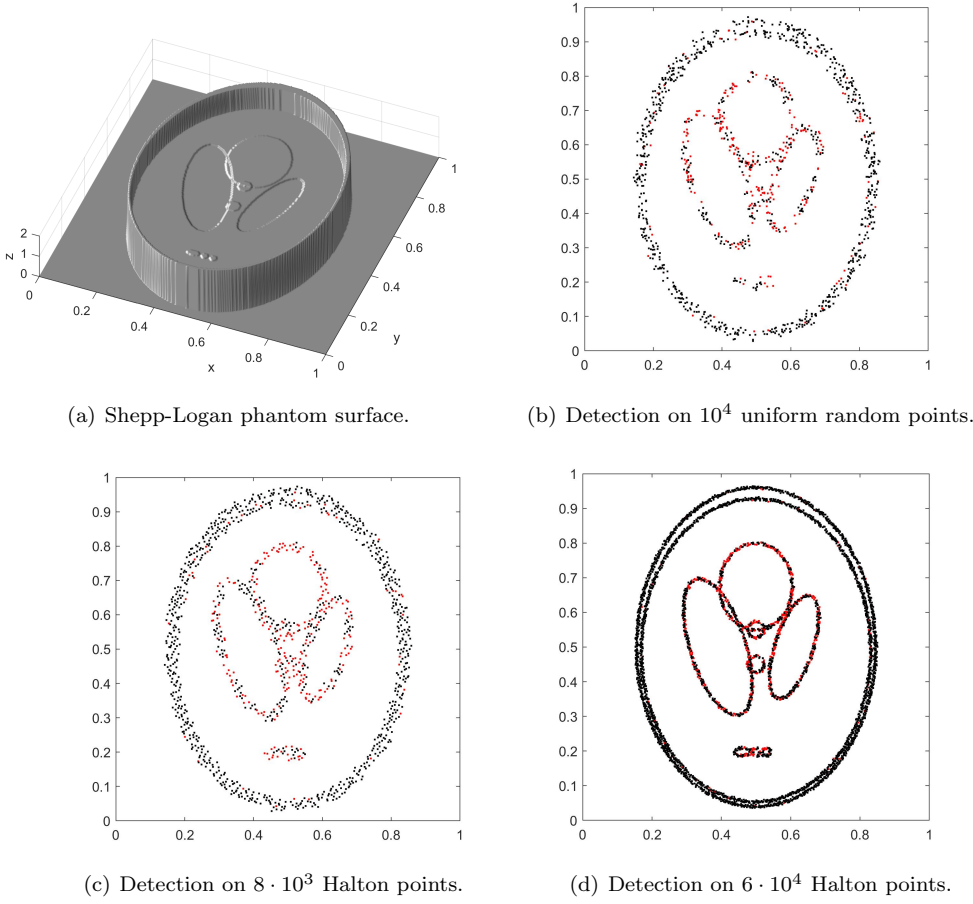
Fig. 3: Application of the detection algorithm on data sampled from the Shepp-Logan phantom surface (top left). The results obtained by considering 10^4 uniformly distributed random points (top right), as well as 8 \cdot 10^3 (bottom left) and 6 \cdot 10^4 (bottom right) Halton points are shown.
