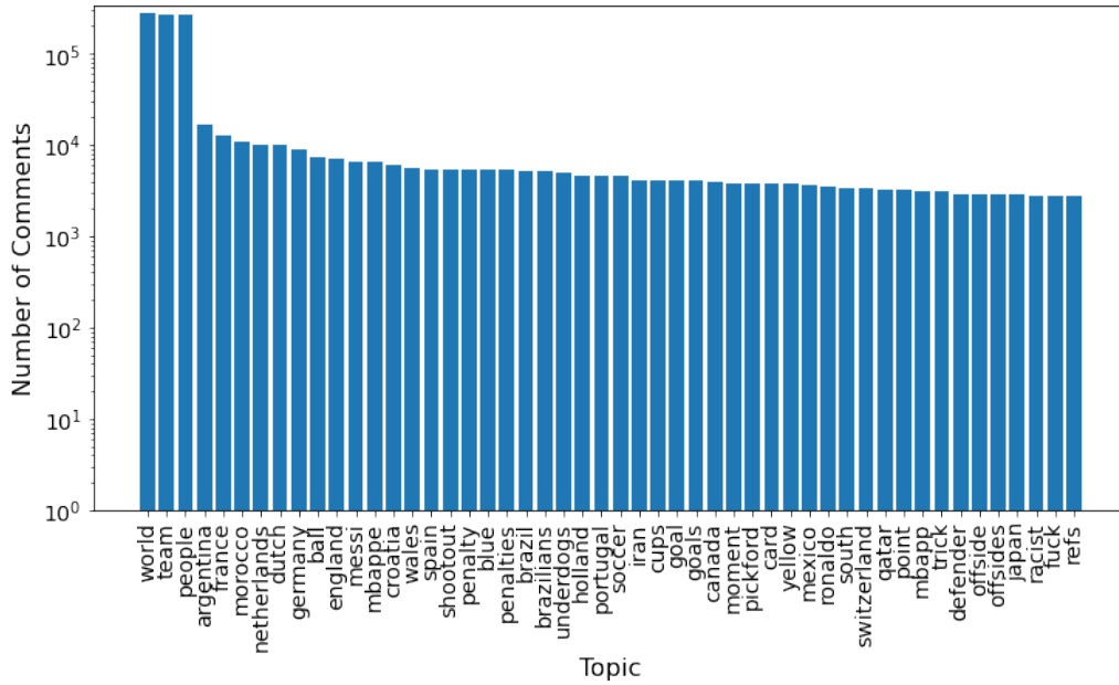
Figure 4: Number of comments per topic (semi-log scale)
