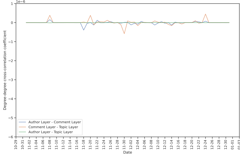
Figure 22: Values of r_{L_1, L_2} for the different pairs of layers over time for the second dataset
