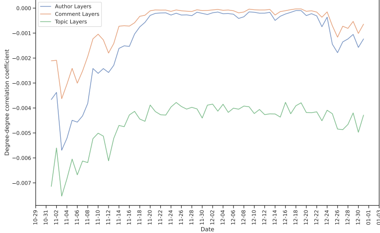
Figure 21: Values of r_L for each layer over time for the second dataset
