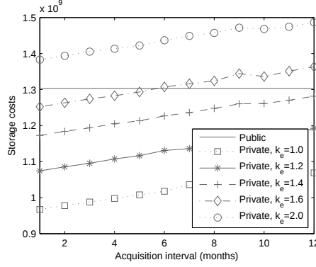
Figure 6: Storage and data transfer costs vs. acquisition intervals for different estimation error levels
