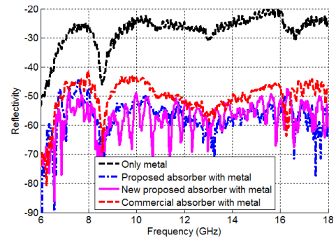
Fig. 14 Comparison of reflectivity of metal, commercial absorber with metal and proposed absorber with metal from Fig. 13.
