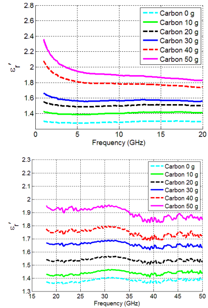
Fig. 10 Real part of the relative complex permittivity ( \epsilon'_r ).
