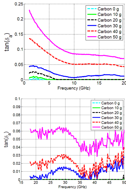
Fig. 12 Alternating electric loss tangent ( \tan(\delta_a) ).
