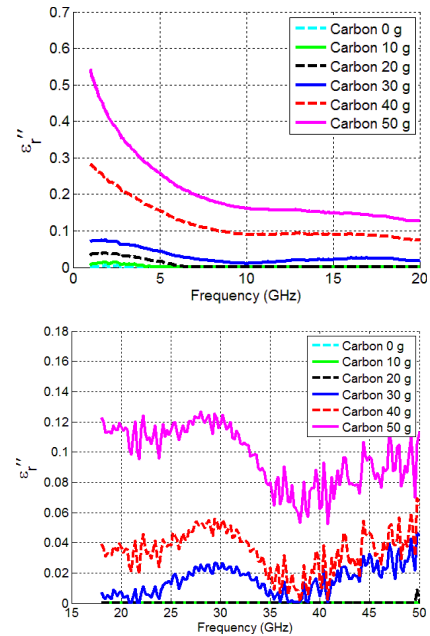
Fig. 11 Imaginary part of the relative complex permittivity ( \epsilon''_r ).
