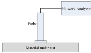
Fig. 9 Dielectric measurement system.
