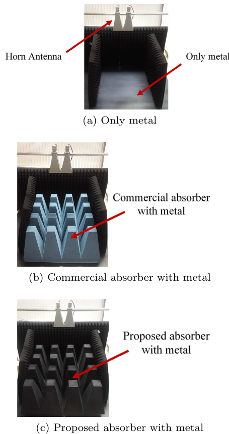
Fig. 13 Measurement setup of reflectivity in frequency 6 GHz to 18 GHz.
