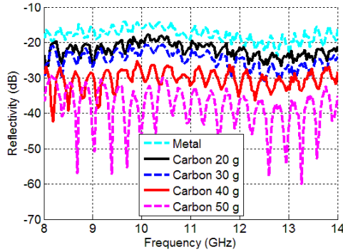
Fig. 2 Comparison of reflectivity of various amount of CCB from 20 to 50 g.
