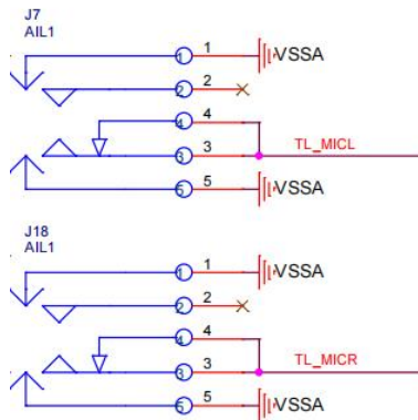
LINE_IN Connection
