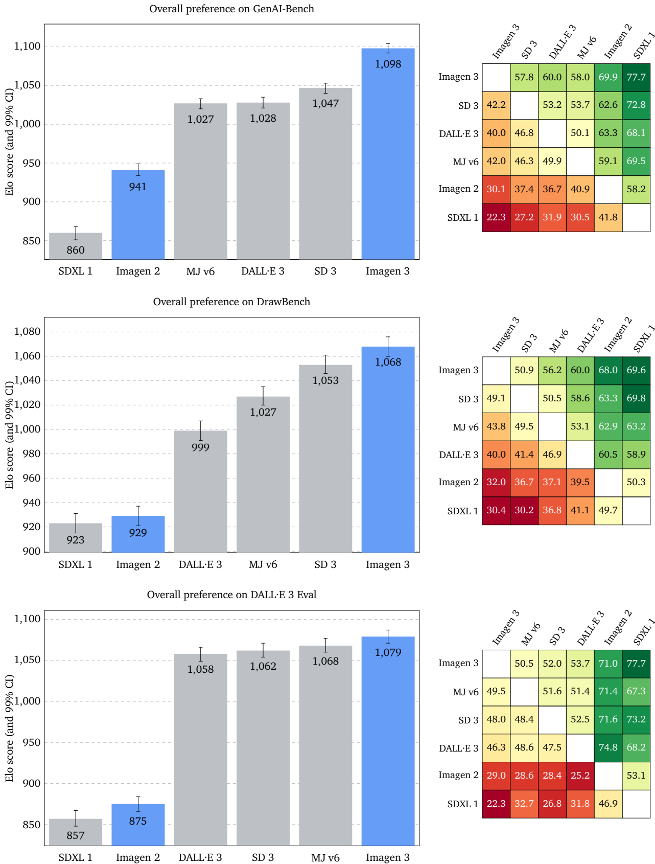
Figure 2 | Overall preference: Elo scores and win-rate percentages on GenAI-Bench, DrawBench, and DALL-E 3 Eval. Please refer to Appendix D for updated human evaluation results as of December 2024.
