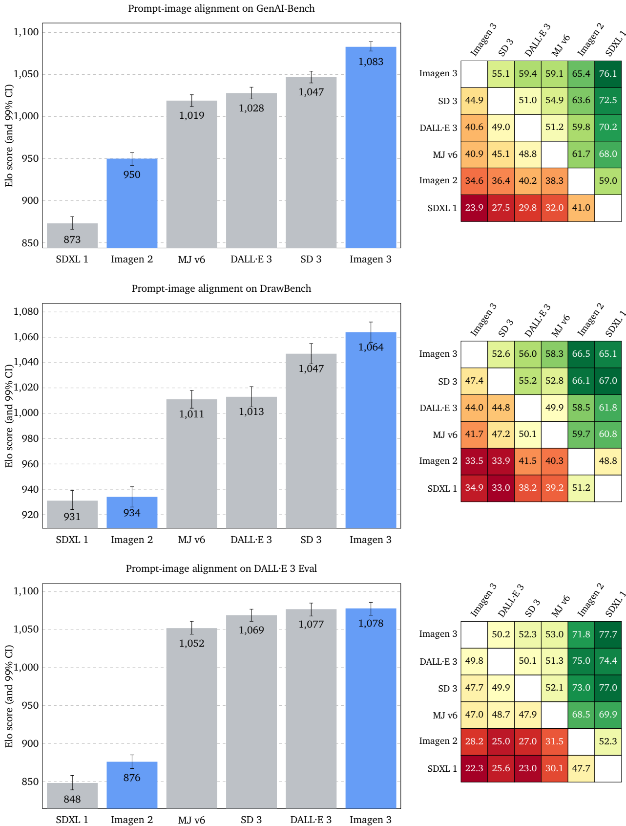
Figure 3 | Prompt-Image Alignment: Elo scores and win-rate percentages on GenAI-Bench, DrawBench, and DALL-E 3 Eval. Please refer to Appendix D for updated human evaluation results as of December 2024.
